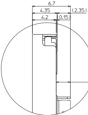
DETAIL B (5:1)
