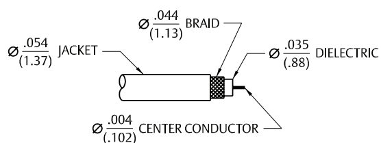
1.37 mm Coaxial Cable
