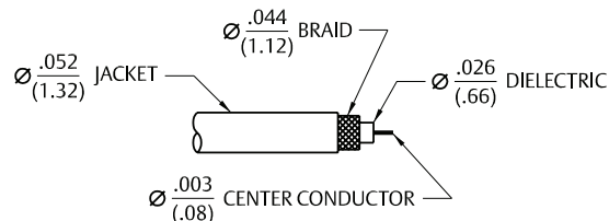
1.32 mm Coaxial Cable
