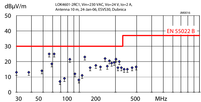
Fig. 9 Radiated disturbances measured according to EN 55011/55032 at V_{i\text{nom}} and I_{o\text{nom}} . LOK4601-2R, V_i = 230 VAC.
