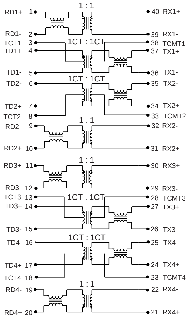
S558-5999-Z3 (Quad Port Dual Stack RJ-45)
