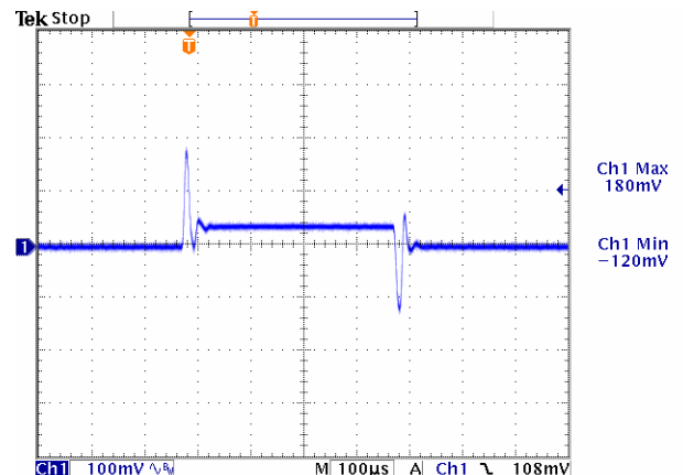
Figure 14. V_{in}=12V , V_{out}=1.0V
