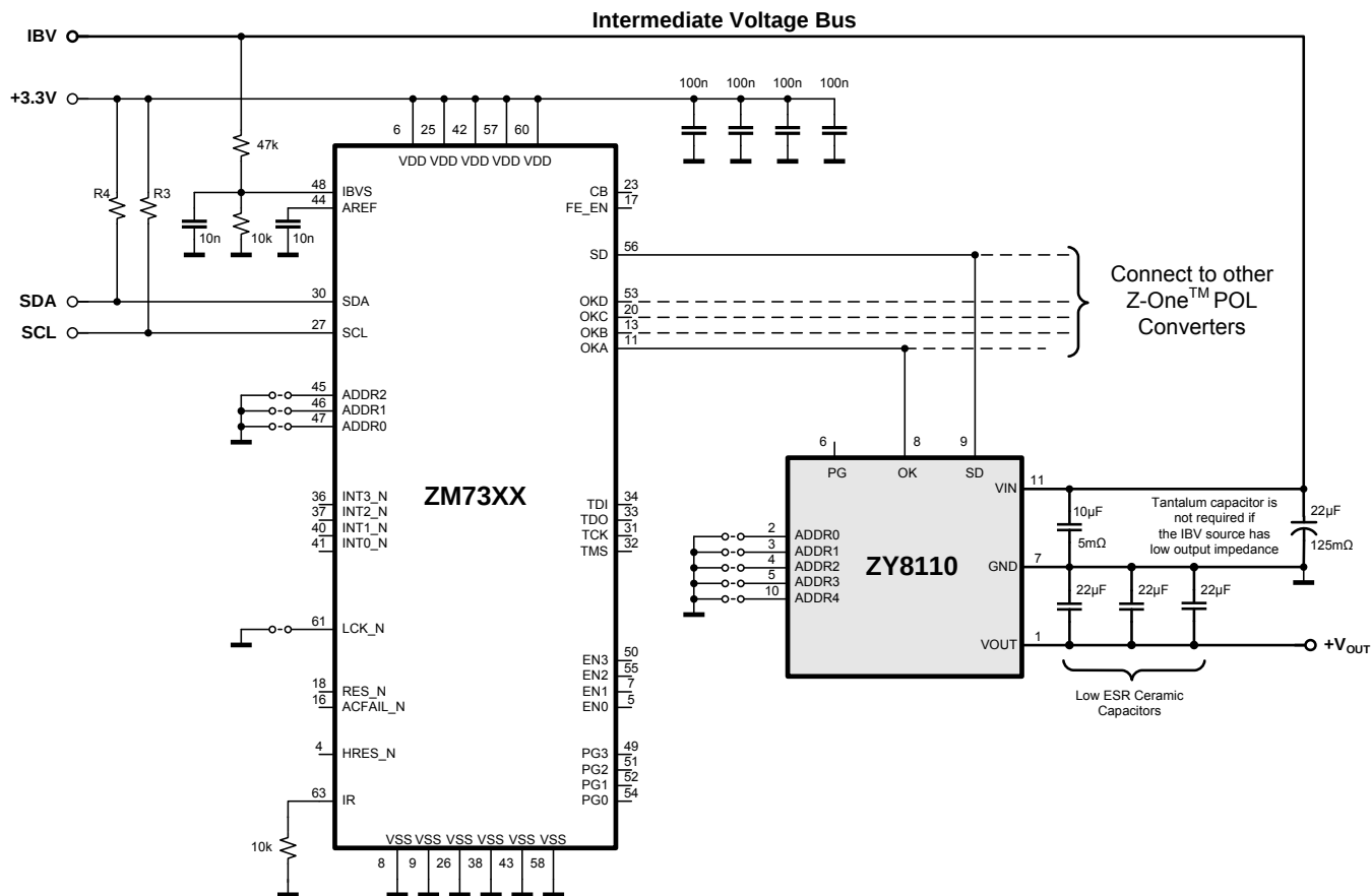
Figure 17. Block Diagram of Typical Application with Digital Power Manager and I 2 C Interface
