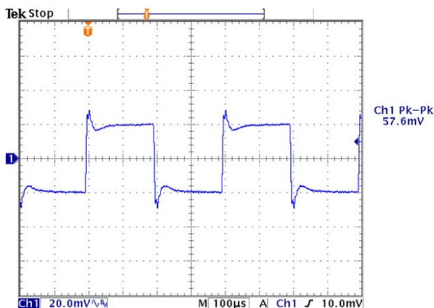
Figure 22. Transient Response with Optimal Voltage Positioning
