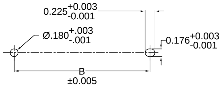
Recommended Mounting Holes
