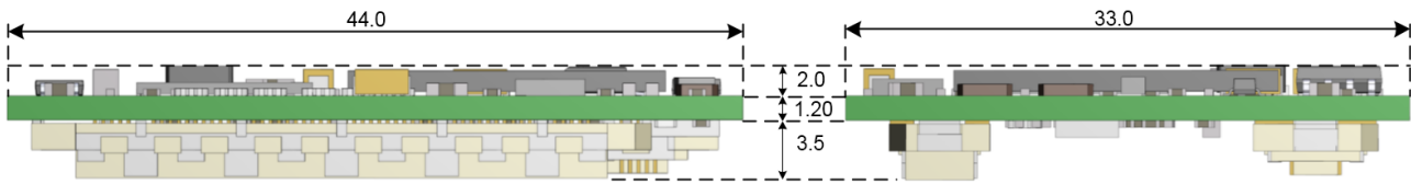
Figure 6.3: Mechanical outline (side view)
