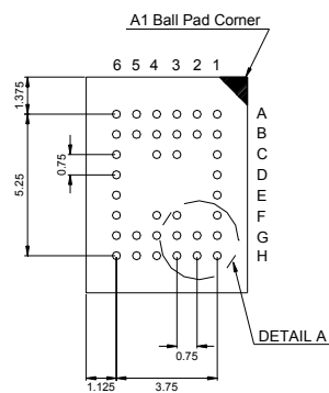
BOTTOM VIEW ( BALL SIDE )
