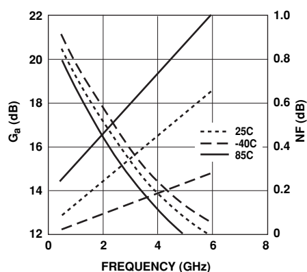
Figure 14. F_{min} and G_a vs. Frequency and Temperature, V_{DS}=2V , I_{DS}=15\text{ mA} .
