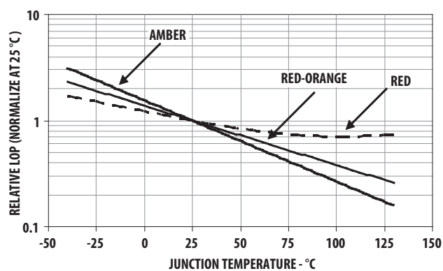
Figure 9. Relative Light Output vs Junction temperature
