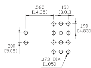
P.C.MOUNTING
