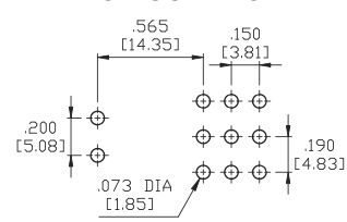
P.C.MOUNTING
