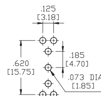
P.C.MOUNTING
