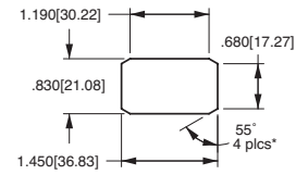
MOUNTING HOLE
