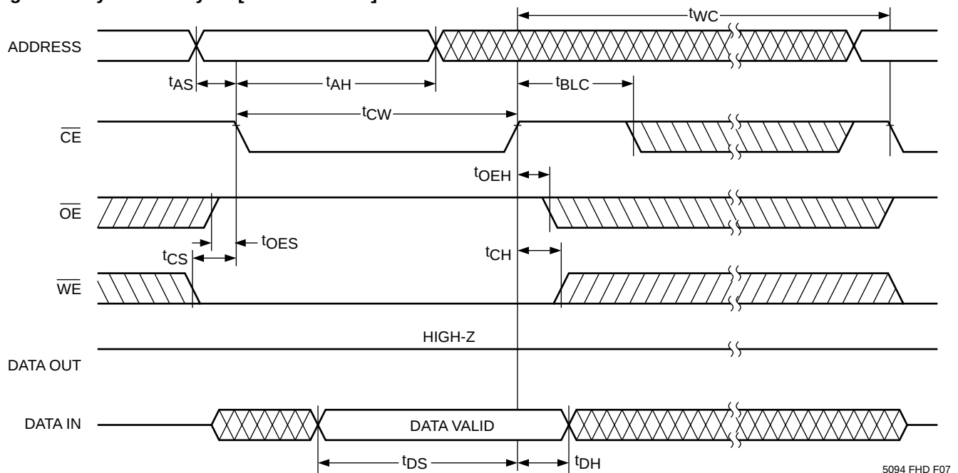
Figure 5. Byte Write Cycle [ \overline{\text{CE}} Controlled]
