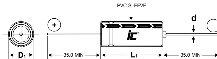
LEAD INFORMATION VS. CASE DIAMETER
