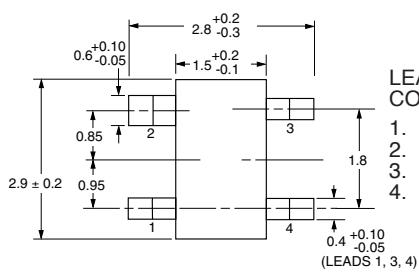
PACKAGE OUTLINE 39R (SOT-143)
