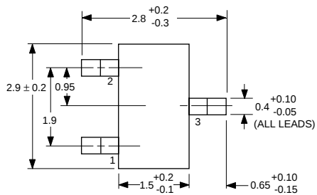
PACKAGE OUTLINE 33
