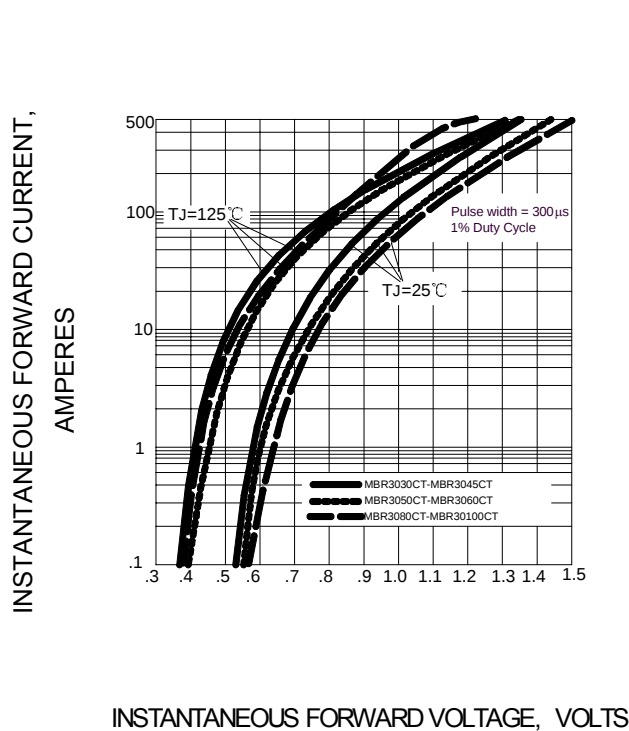
FIG.3 – TYPICAL FORWARD CHARACTERISTIC
