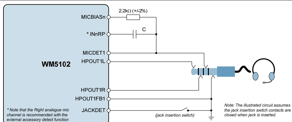
Figure 91 External Accessory Detection
