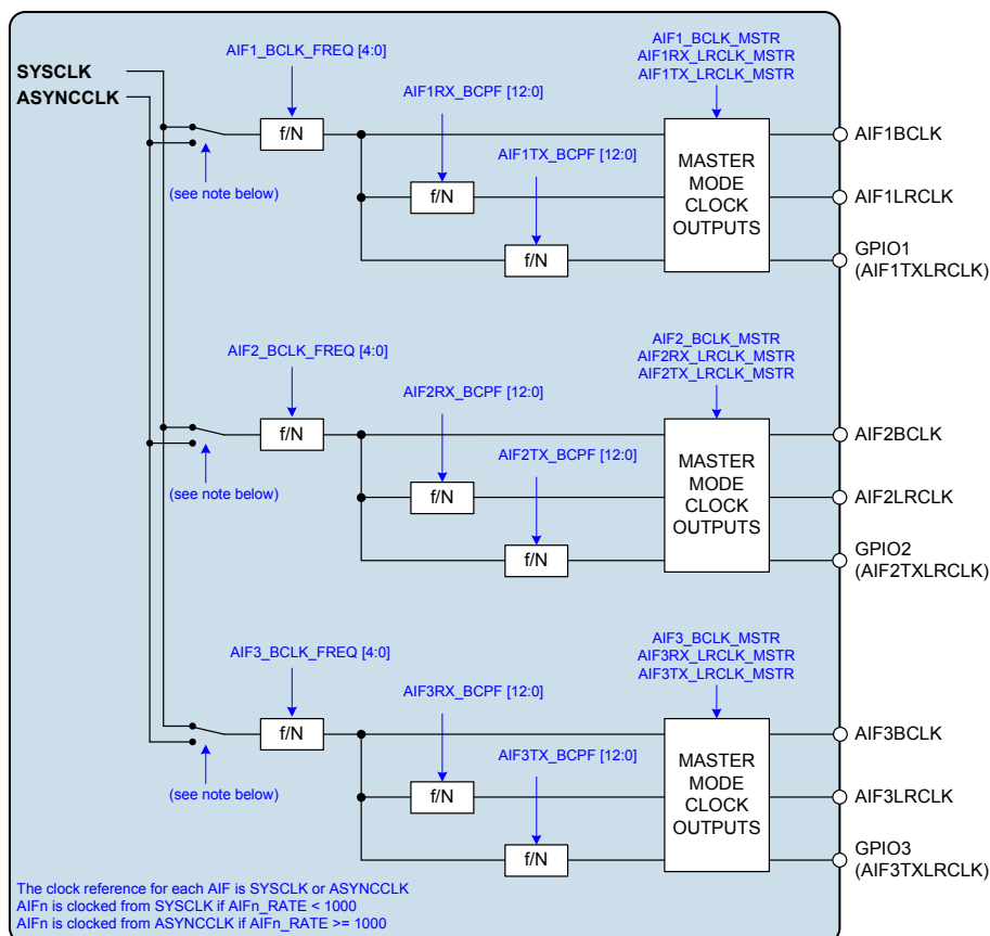
Figure 69 BCLK and LRCLK Control
