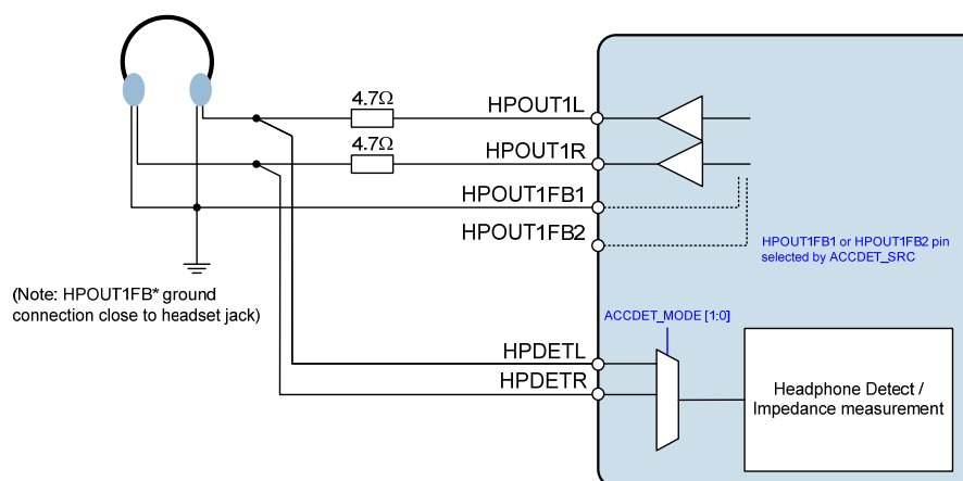
Figure 66 Headphone Detect Interface
