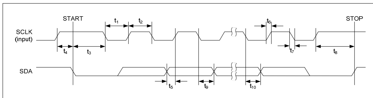
Figure 9 Control Interface Timing - 2-wire (I2C) Control Mode
