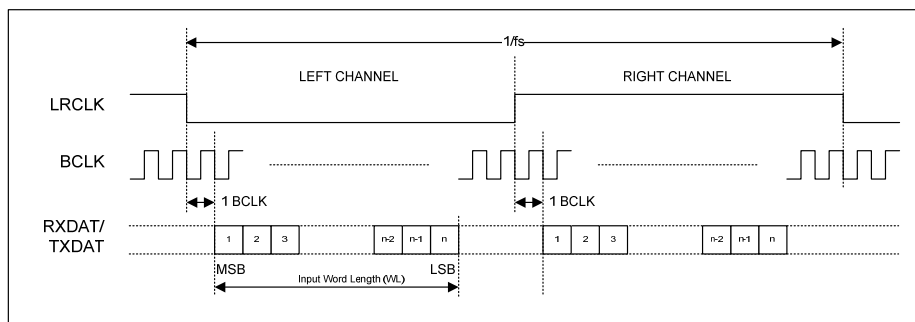
Figure 47 I2S Data Format (assuming n-bit word length)
