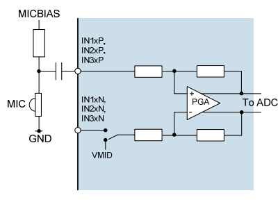
Figure 14 Single-Ended ECM Input
