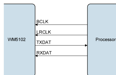
Figure 44 Slave Mode
