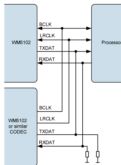
Figure 54 TDM with Other CODEC as Master
