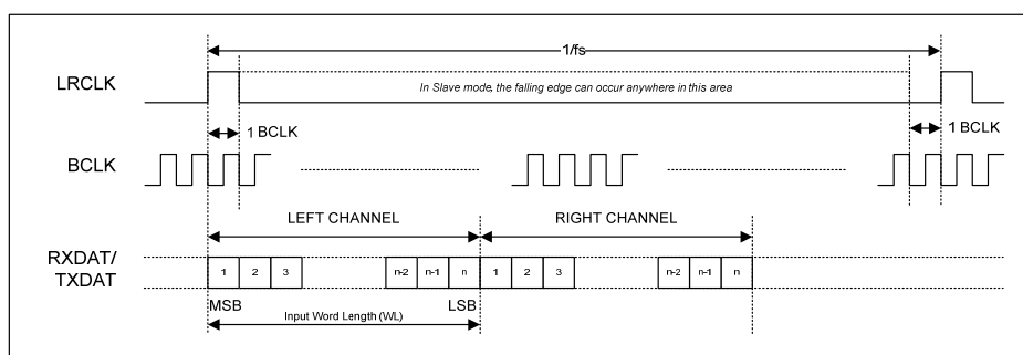
Figure 46 DSP Mode B Data Format
