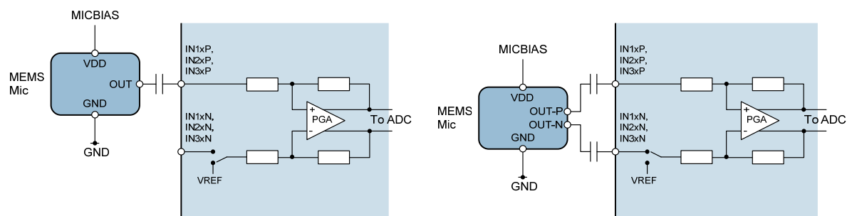
Figure 84 Single-Ended and Differential Analogue Microphone Connections
