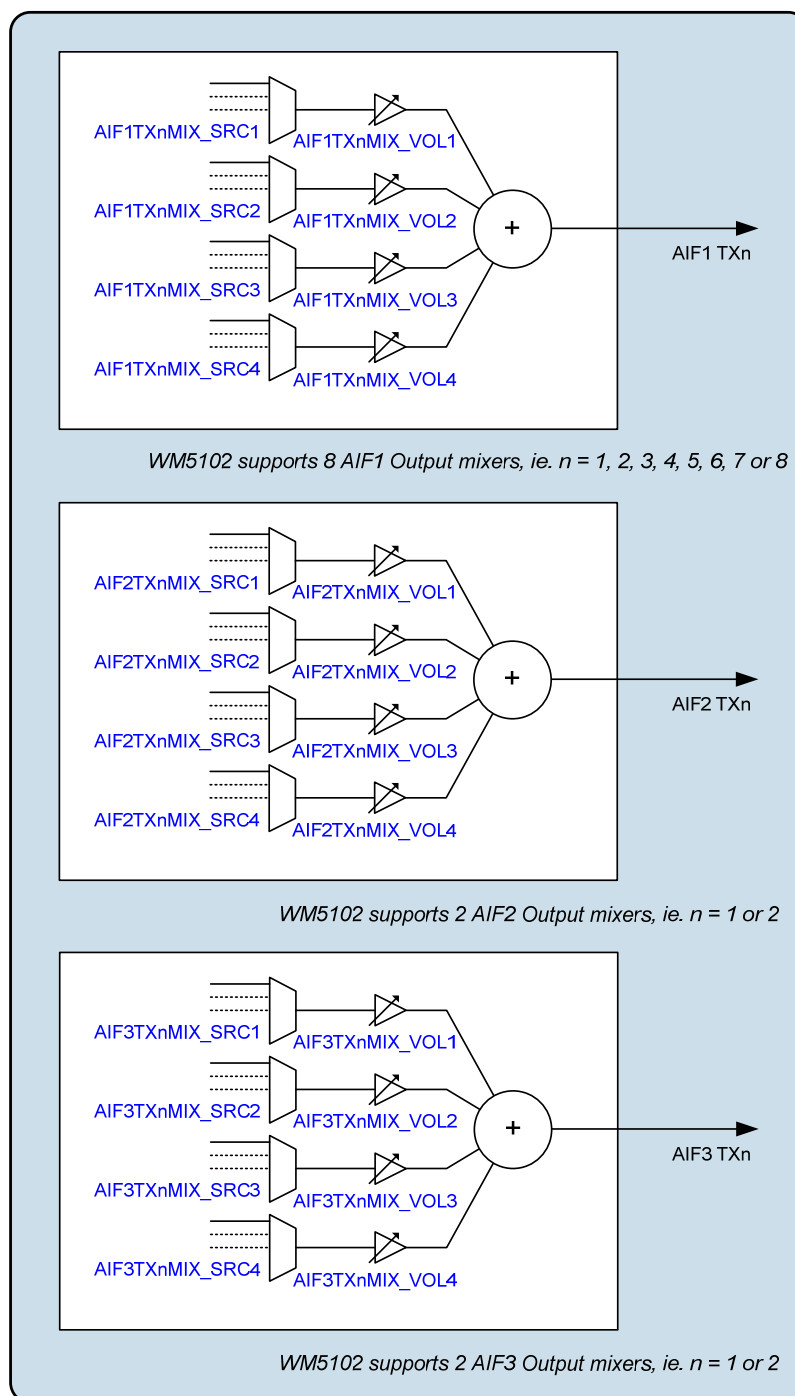
Figure 25 Digital Core AIF Outputs
