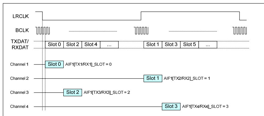
Figure 51 I2S Example
