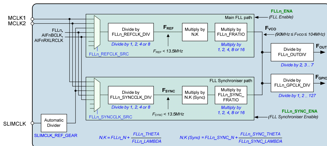
Figure 70 FLL Configuration
