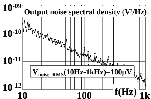
Figure 8: S_{Vout}(V^2/Hz) @ 25^\circ C , I_{Load}=100mA
