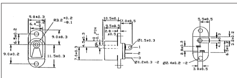
DC-13 panel mounting pin / ring type with switch. Rated 12V / 5A. DC-13A with 2.1mm dia. pin. DC-13B with 2.5mm dia. pin. DC-13A (FC681492) DC-13B (FC681493)
