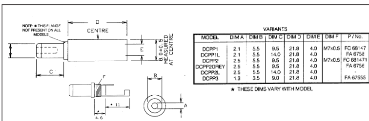
DCP1 DC Line connector. Rated 12V / 5A. DCP1 with 2.1mm dia. pin. DCP2 with 2.5mm dia. pin.
