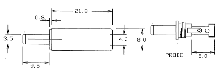
DCP3 DC Line connector. Rated 12V / 5A. With 1.3mm dia. pin
