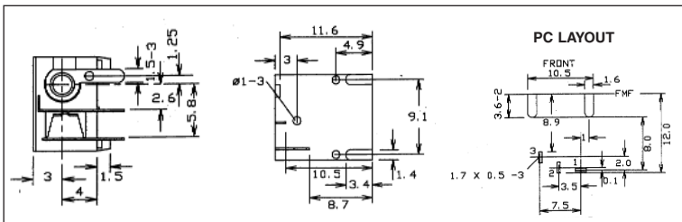
DC-12A PCB mounting pin / ring type with switch. Rated 12V / 5A. With 2.1mm dia. pin.
