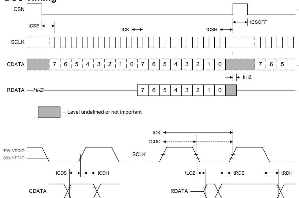
Figure 113 C-BUS Timing
