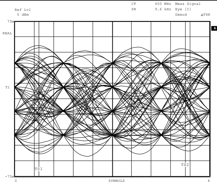
Eye Diagram
