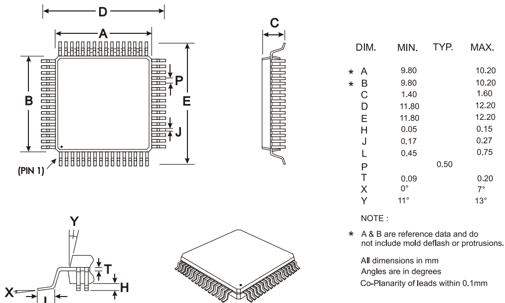
Figure 115 Mechanical Outline of 64-pin LQFP (L9)
