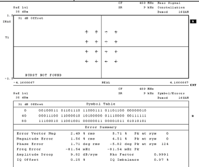
Error Vector
