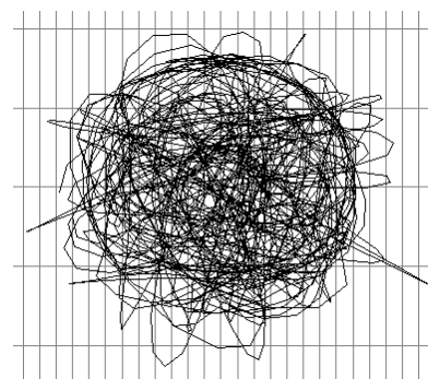
Figure 27 Constellation Diagram – frequency error
