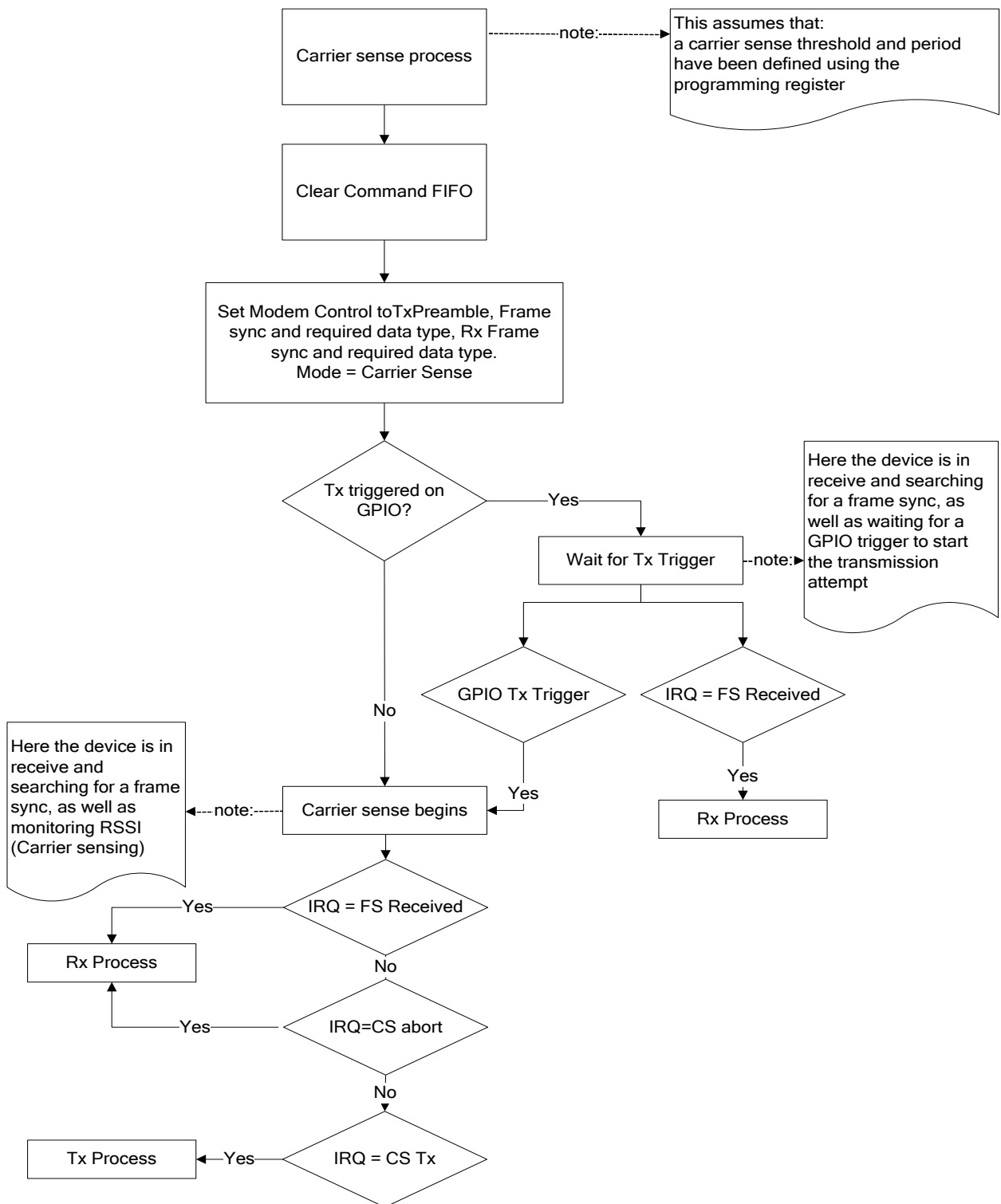
Figure 19 Carrier Sense
