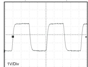
CMOS Output Waveform
