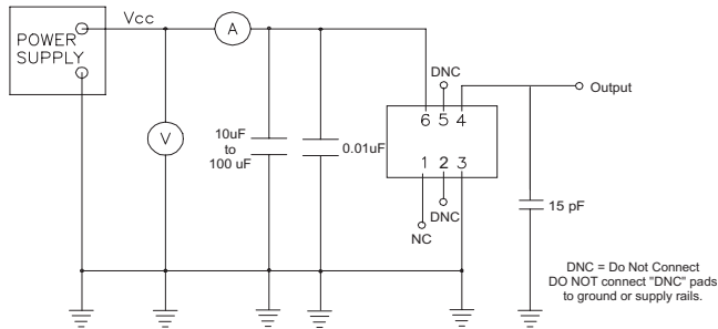
LVC MOS Test Circuit
