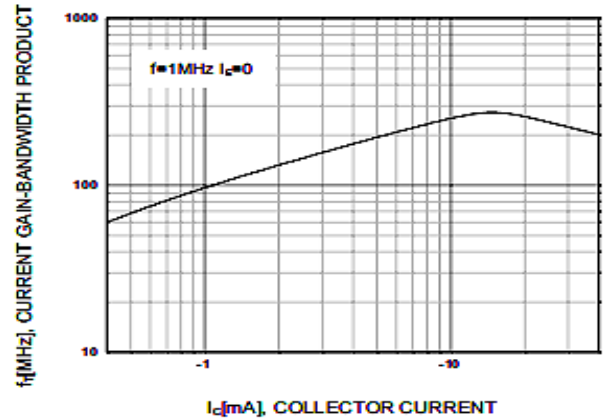
Fig 6: Current Gain Bandwidth Product
