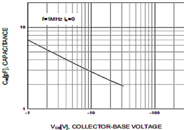
Fig 3: Collector Output Capacitance
