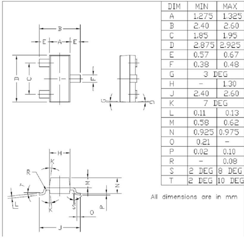
SOT-23 Leaded Plastic Package
