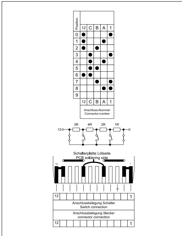
Code 731 BCD positive + complement - make before break contact
