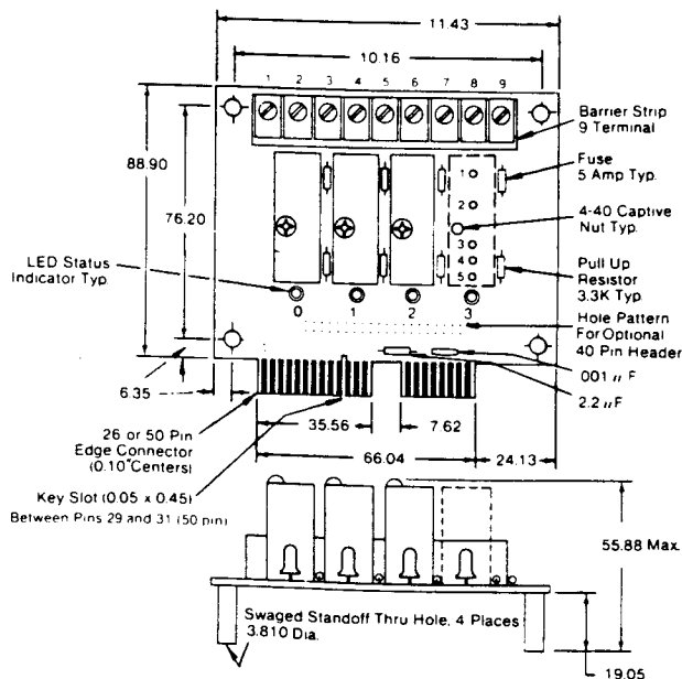
MS-4H Mounting Board
