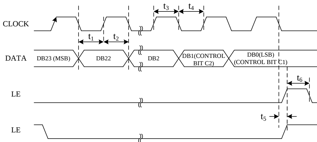
Figure 1. Timing Diagram
