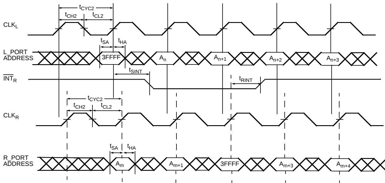
Figure 23. MailBox Interrupt Timing [59, 60, 61, 62, 63]
