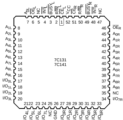
Figure 2. Pin Diagram - PLCC (Top View)
