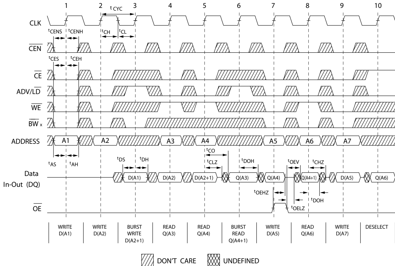
Figure 7. Read/Write/Timing [24, 25, 26]
