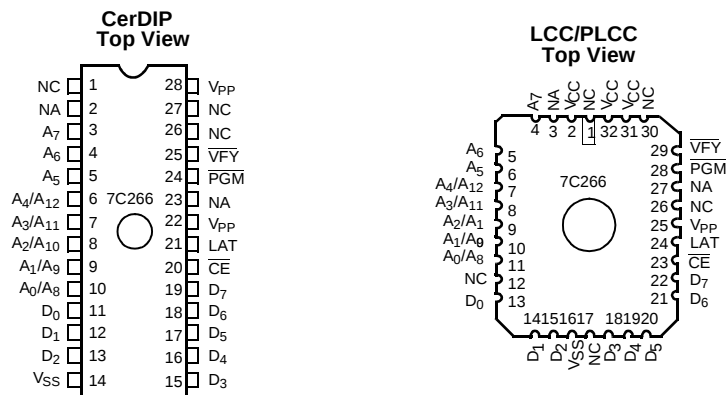
Figure 1. Programming Pinout
