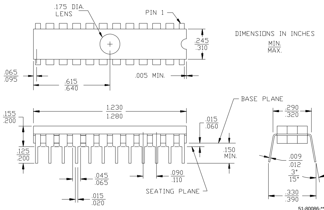
24-Lead (300-Mil) Windowed CerDIP W14
