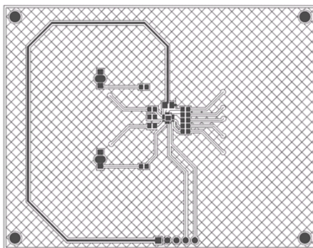
Figure 9. Bottom Layer
