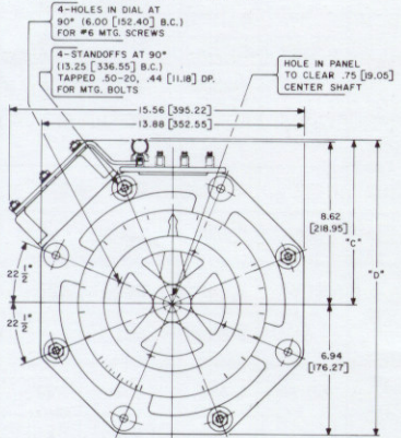
PANEL MOUNTED
