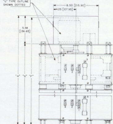
MOTOR DRIVEN
