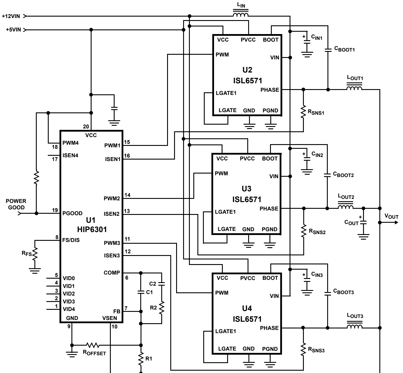
FIGURE 3. TYPICAL APPLICATION
