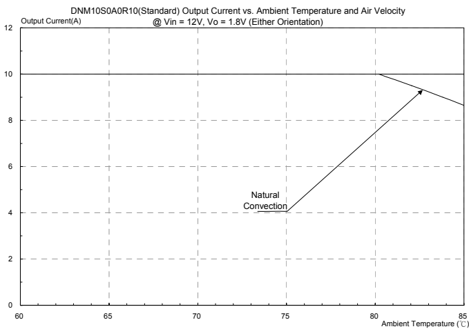
Figure 33: DNM10S0A0R10(Standard) Output current vs. ambient temperature and air velocity @ Vin=12V, Vo=1.8V(Either Orientation) DS_DNM10SIP10_03062009
