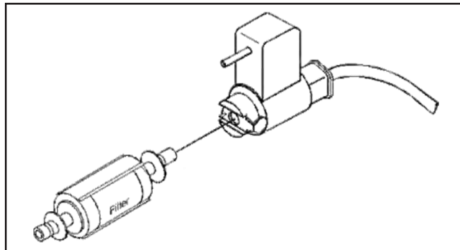
Figure 7: Inserting the disposable filter
