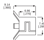
SPEED CLIP 515-0051
