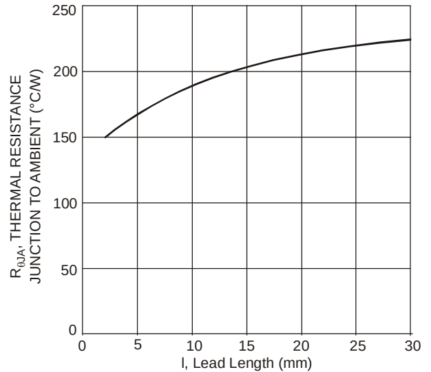
Fig. 2 Typical Thermal Resistance vs. Lead Length
