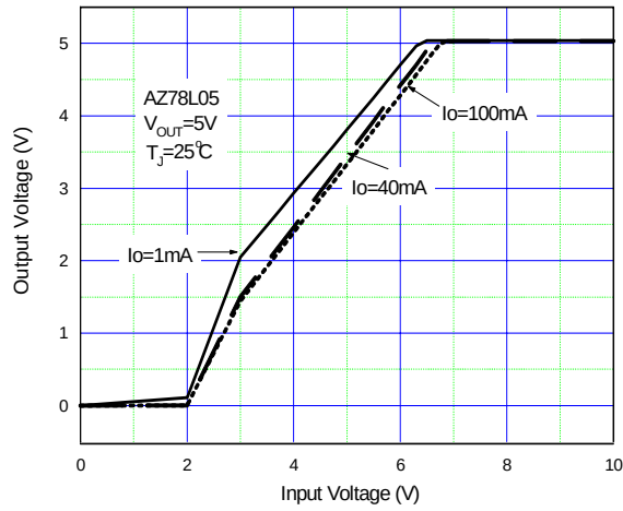
Figure 4. Dropout Characteristics
