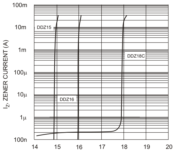
Fig. 6 Typical Reverse Characteristics, DDZ15 - DDZ18C
