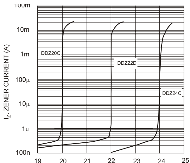
Fig. 7 Typical Reverse Characteristics, DDZ20C - DDZ24C
