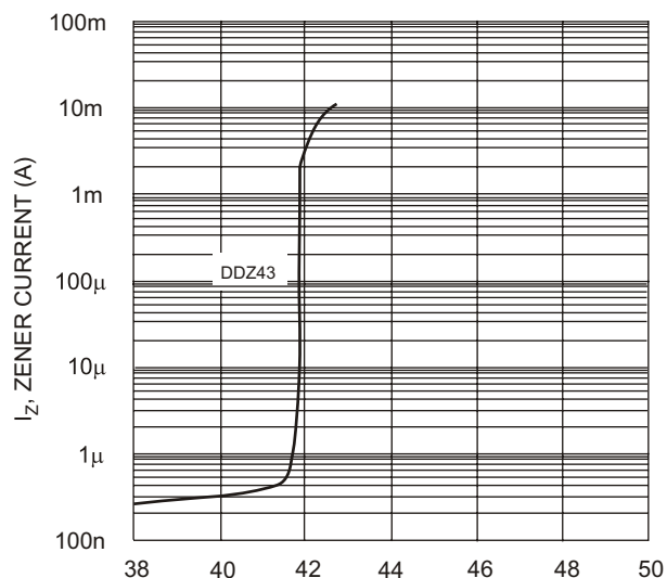
Fig. 9 Typical Reverse Characteristics, DDZ43
