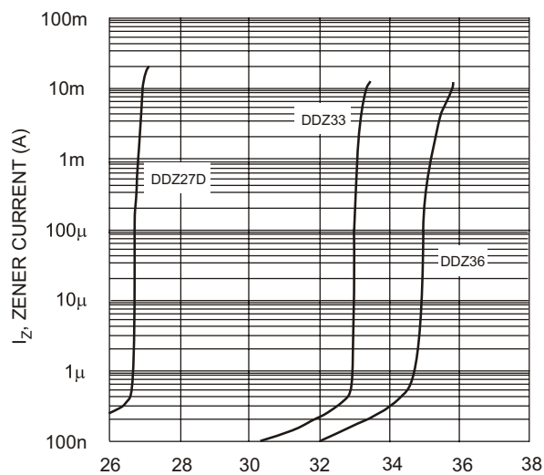
Fig. 8 Typical Reverse Characteristics, DDZ27D - DDZ36
