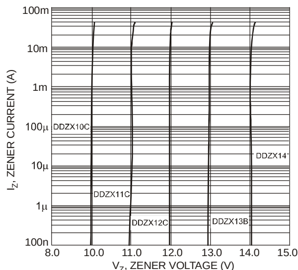
Fig. 5 Typical Zener Breakdown Characteristics DDZX10C - DDZX14
