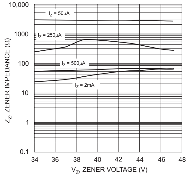
Fig. 14 Typical Zener Impedance Characteristics, DDZX36TS - DDZX43TS
