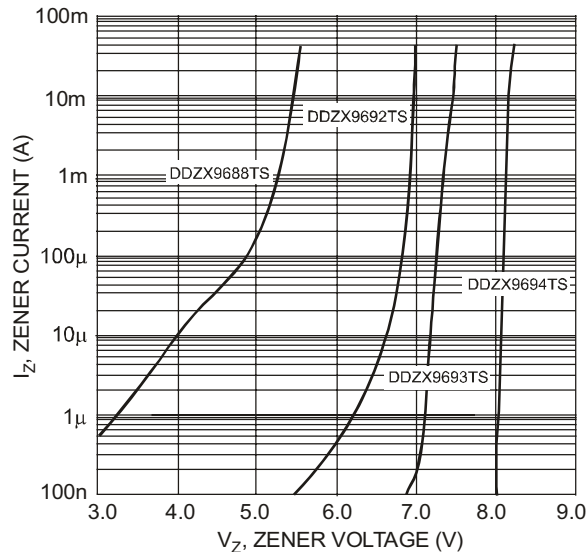
Fig. 4 Typical Zener Breakdown Characteristics DDZX9688TS - DDZX9694TS
