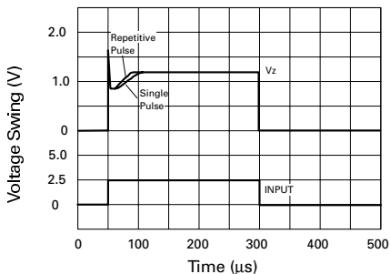
Pulse Response
