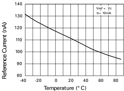
Reference Current v Temperature
