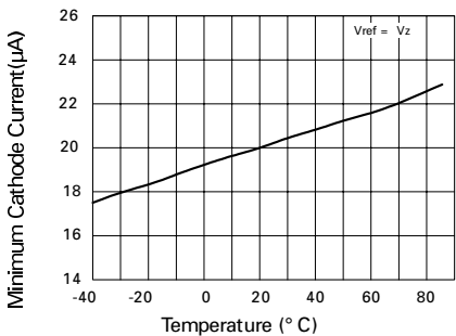
Cathode Current v Temperature
