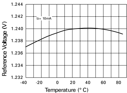
Reference Voltage v Temperature
