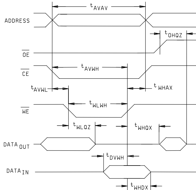
Timing waveform of write cycle number 1 ( \overline{\text{WE}} controlled timing) (see notes 1, 2, 3, 6, and 7)
