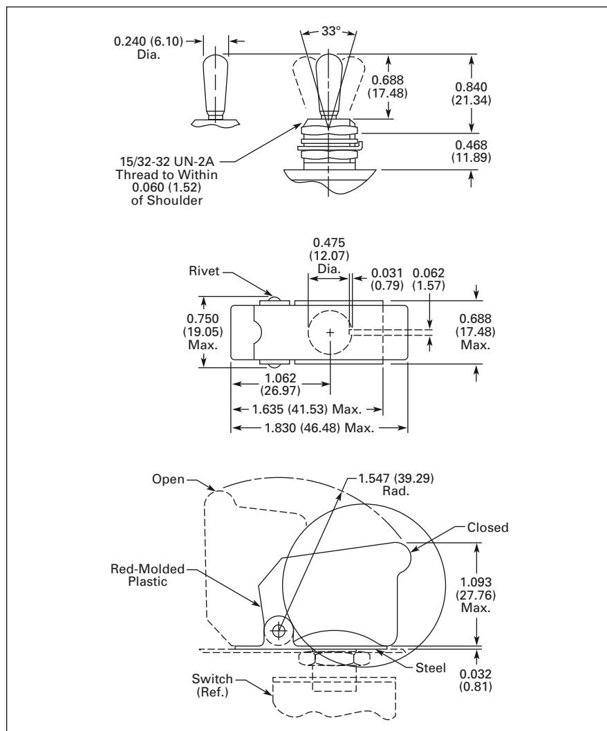
Figure 47-8. Switch Guard— Approximate Dimensions in Inches (mm)
