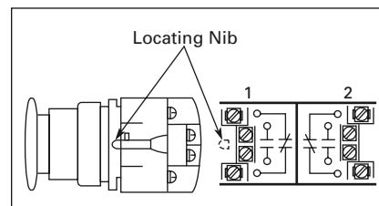
Figure 47-145. Locating Nibs
