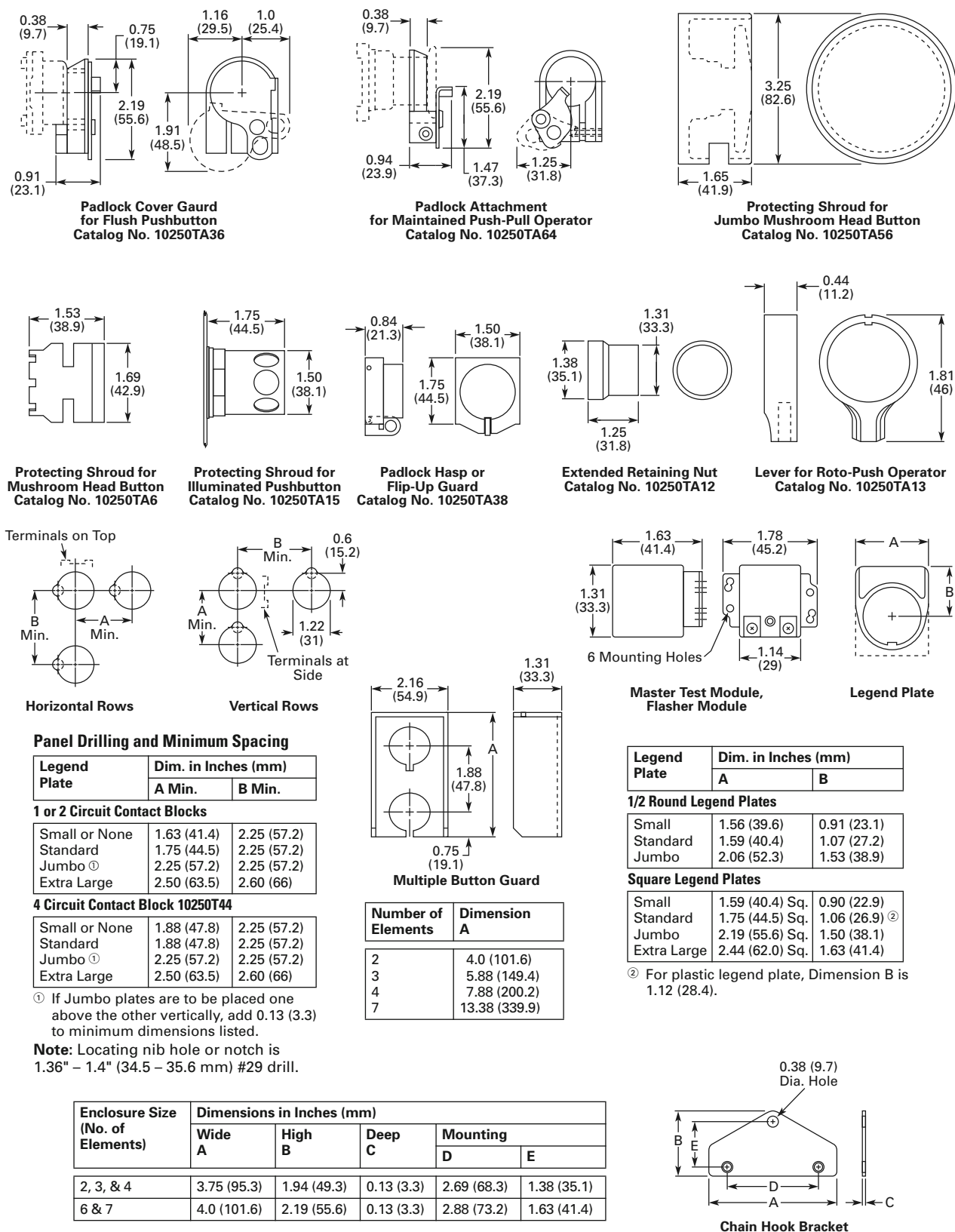
Figure 47-121. Approximate Dimensions in Inches (mm)
