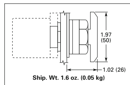
Figure 47-47. E22/EM22 Series 50 mm Dia. Push-Pull Button
