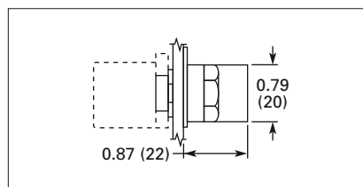
Figure 47-70. E22 Series 3-Position — 60° Throw — Knob
