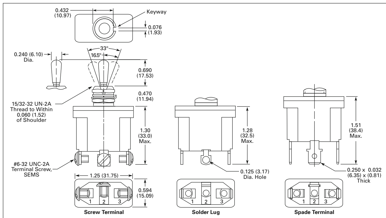
Figure 47-6. One-Pole Econoswitch E10E Series Toggle Switches — Approximate Dimensions in Inches (mm)
