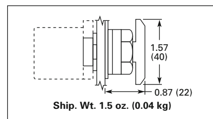
Figure 47-46. E22/EM22 Series 40 mm Dia. Push-Pull Button
