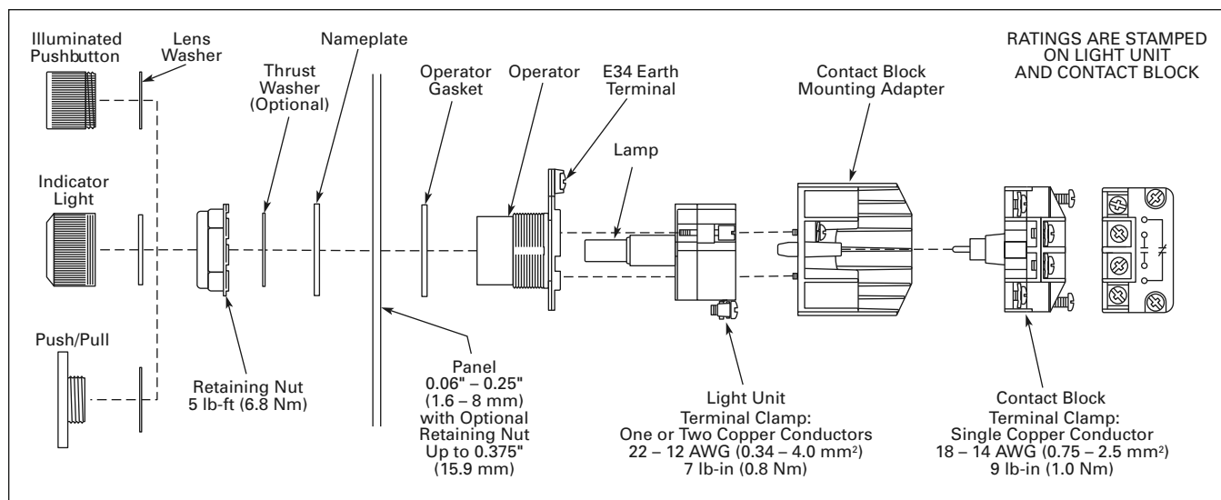
Figure 47-154. Operator Assembly
