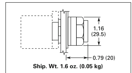
Figure 47-35. E22/EM22 Series 25 mm Dia. Extended Lens
