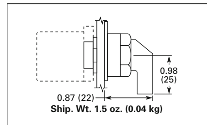
Figure 47-71. EM22 Series — 60° Throw — Lever
