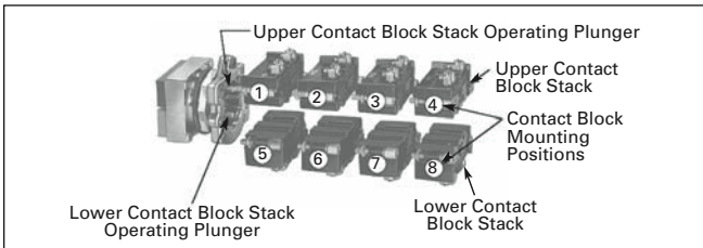
Figure 47-83. Mounting Positions
