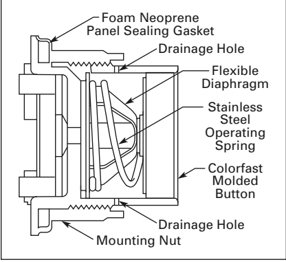
Figure 47-123. Diaphragm Seal
