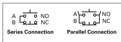
Figure 47-110. Series and Parallel Connection
