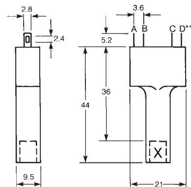
Terminal Arrangement
