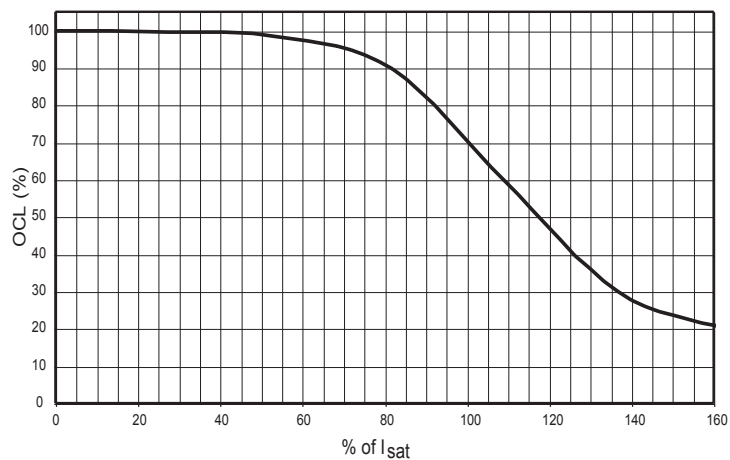
OCL vs I_{sat} DR73
