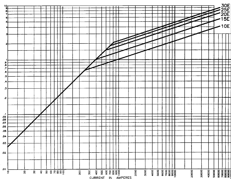
Max. Peak Let-Through Current Curves
